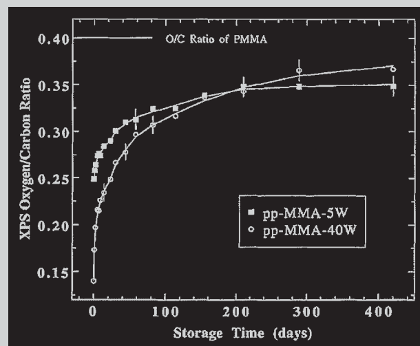
XPS O/C ratios ( O^{1s} emission) as a function of storage time, of plasma-polymerized methyl methacrylate deposited at power levels of 5 and 40 W.
