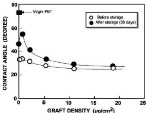
Figure 10. Variation of CA with grafting density of acrylic acid on PET films. Reproduced with permission from ref. [99]
