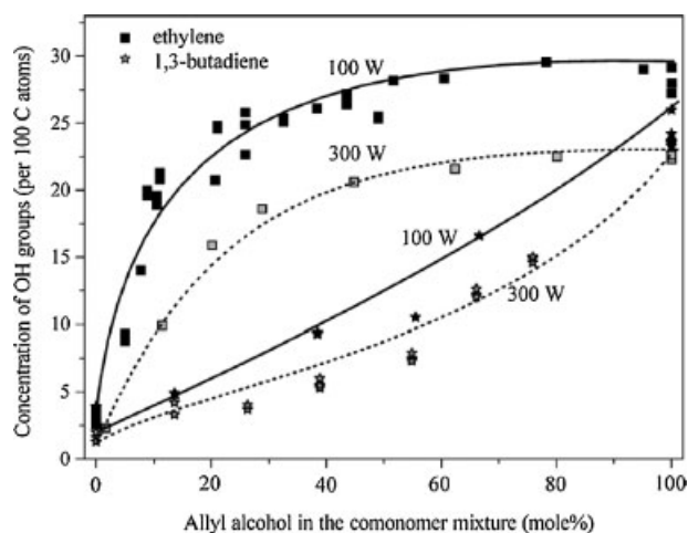
Figure 5. Densities of OH groups on ethylene/allyl alcohol and butadiene/allyl alcohol copolymers measured by XPS and derivatization with TFSA. Reproduced with permission from ref. [144]
