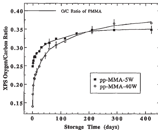
Figure 9. XPS O/C ratios (O 1s emission) as a function of storage time, of plasma-polymerized methyl methacrylate deposited at power levels of 5 and 40 W. Also included is the theoretical value of O/C for PMMA (0.4). Error bars represent one standard deviation. Reproduced with permission from ref. [118]
