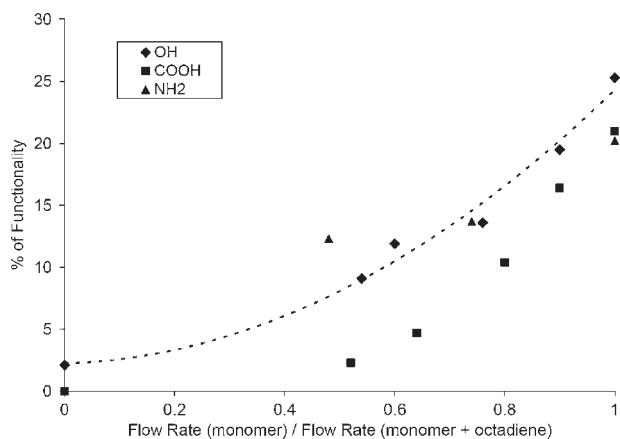
Figure 6. Densities of OH groups on octa-1,7-diene/allyl-alcohol plasma polymer derivatized with TFAA and measured by XPS. The line is drawn for illustration only, to connect the percentage of OH groups with respect to different ratios of flow rates. Data from ref. [43] and [154].
