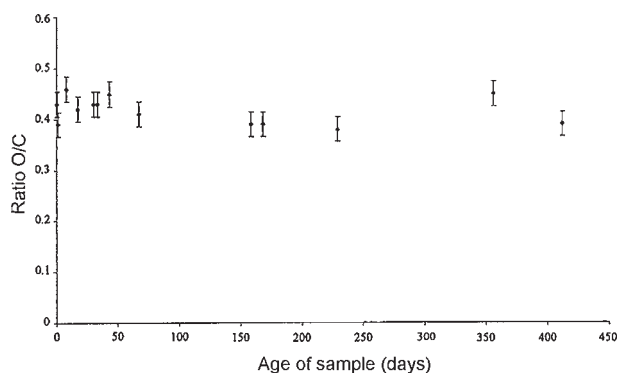
Figure 8. O/C ratio of acrylic acid plasma polymer as a function of sample age. Reprinted with permission from ref. [116]
